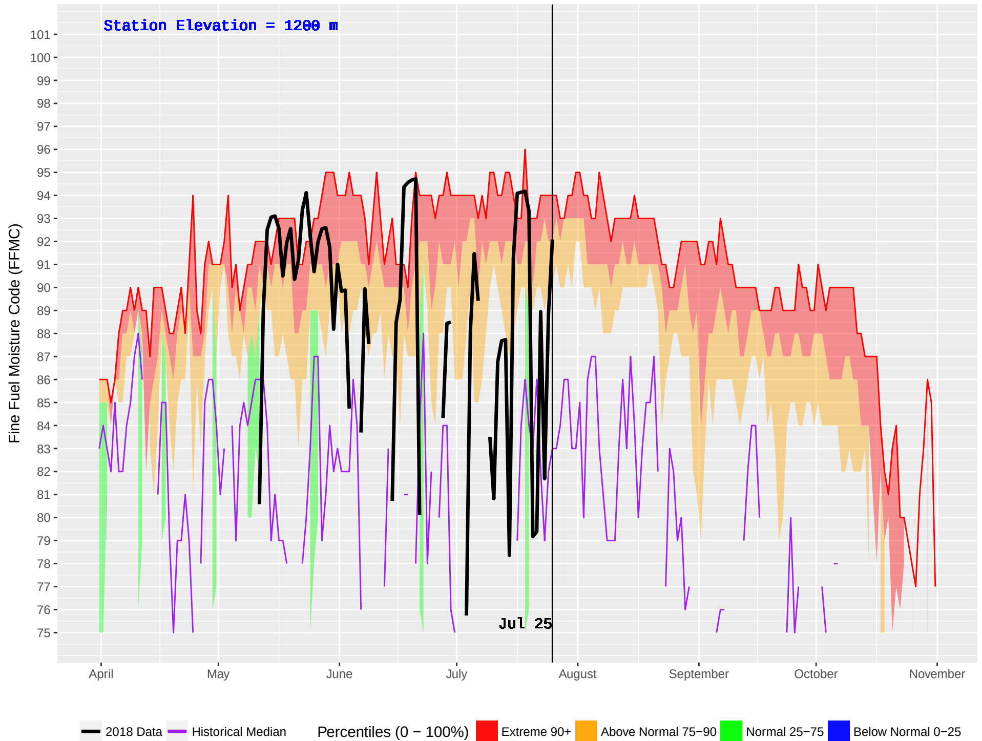
TSAR CREEK (361) : Historical (1986–2016) and Current (2018) Noon Fine Fuel Moisture Code (FFMC)
