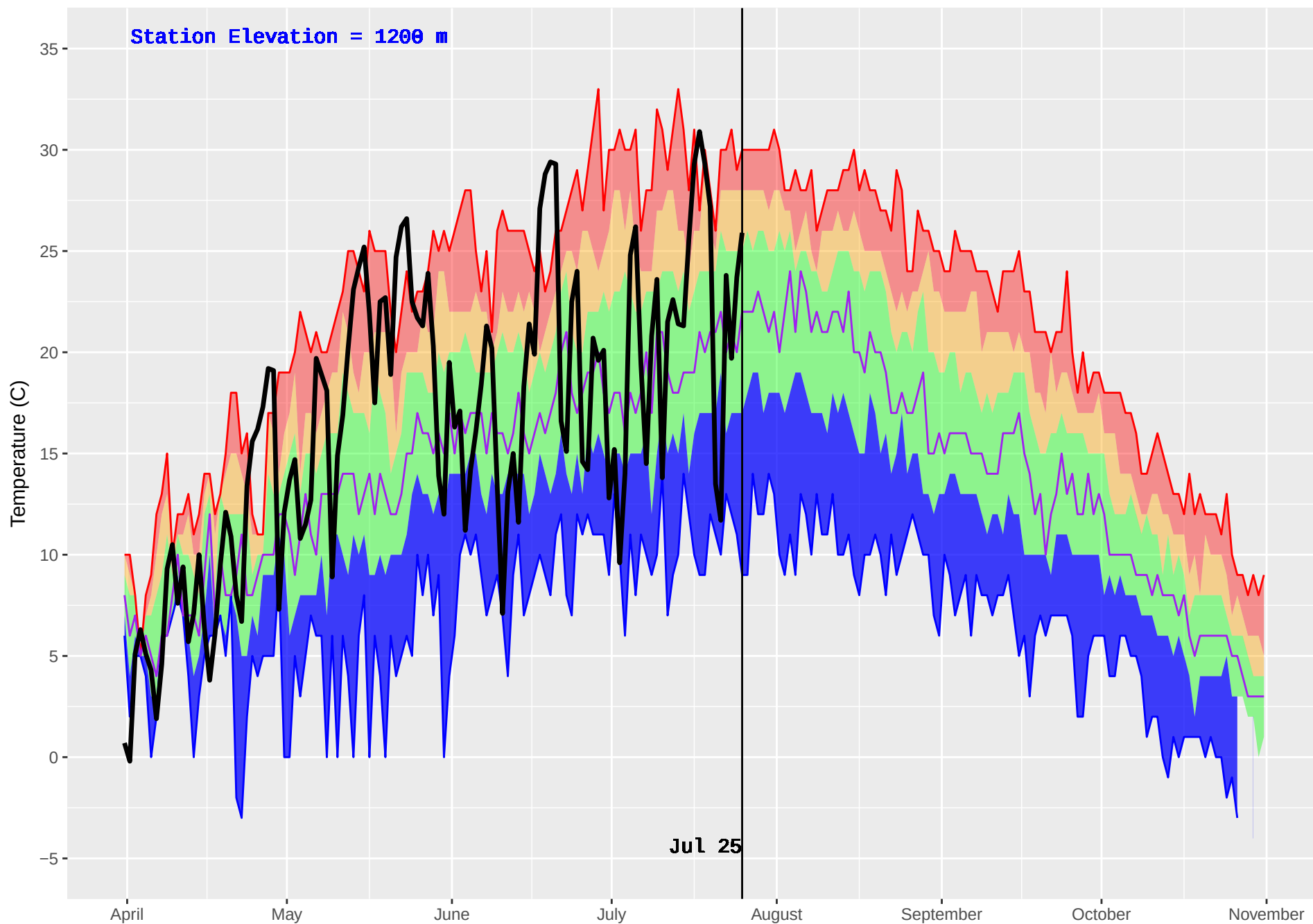
TSAR CREEK (361) : Historical (1986–2016) and Current (2018) Noon Temperature
